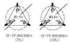
Tripod Wheel Base (Footprint)
